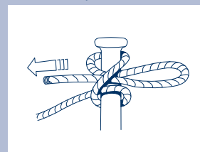
Quick release clove hitch (for short stops)
